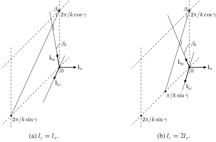
FIGURE 2. Wave Cartesian coordinates ( k and \gamma as in Figure 1.) For l_z = 0 , see Figure 1, since then \eta_\ell = y and \zeta_\ell = z .
