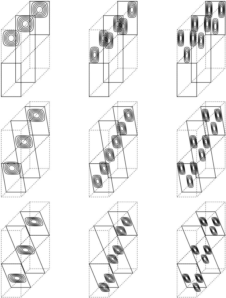
FIGURE 3. Stream-lines of poloidal fields with stream-functions -\kappa_\ell p_n(x) \sin \kappa_\ell \eta t . Here l_z = 0, 1, 2 by row and n = 0, 1, 2 by column; l_y = 1 in all; k and \gamma as in Figures 1 and 2. Only stream-lines corresponding to ‘positive’ rolls of a single period cell are shown; counterrotating rolls are symmetrically disposed. Stream-lines lie in the planes \zeta_\ell = 0, \pi \cos \beta_\ell / k \sin \gamma, 2\pi \cos \beta_\ell / k \sin \gamma , as marked by solid lines. Dashes mark boundaries of two yz -period cells and |x| = 1 .
